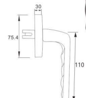
FZD-22HU Material: aluminum alloy+zinc alloy Type: Left and right
