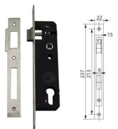
FZD-02B Stainless steel panel zinc alloy locking tongue iron shell
