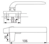
FZD-19WH Material: Aluminum alloy
