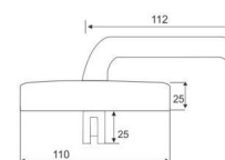
FZD-23HU Material: Zinc alloy
