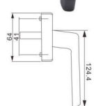
FZD-27HU Material: Zinc alloy+plastic
