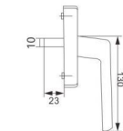
FZD-24ZHU Material: Aluminum alloy+zinc alloy
