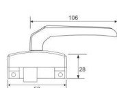
FZD-16HU (Square) Material: Aluminum alloy
