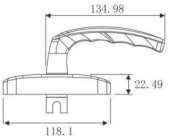
FZD-04HU Material: Aluminum alloy
