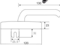
FZD-08HU Material: Aluminum alloy semi zinc aluminum
