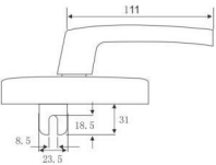
FZD-02HU Material: Aluminum alloy
