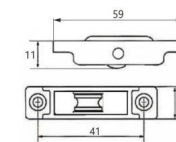
FZD-35R Material: Iron
