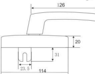
FZD-09HU Material: Aluminum alloy
