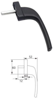
FZD-28HU Material:Aluminum alloy
